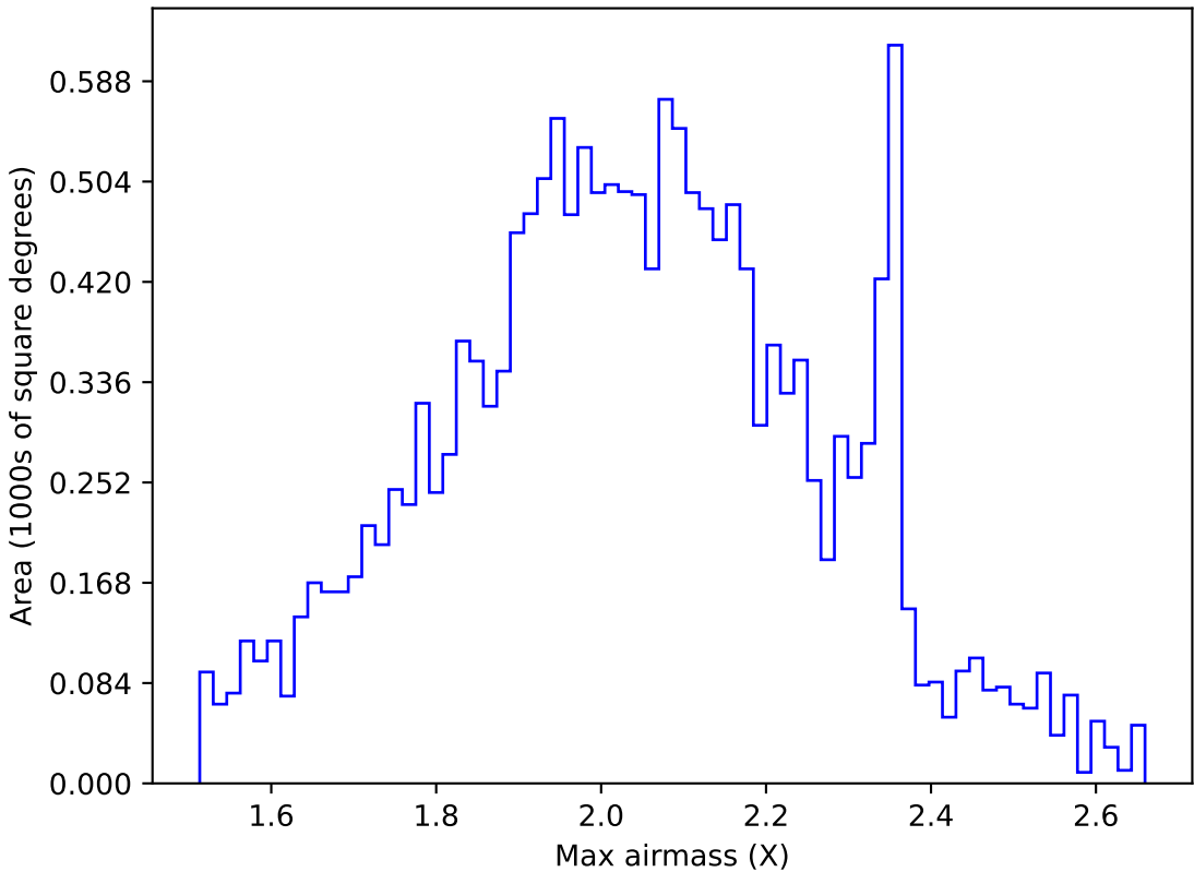
too_combined_no_nss_s10.0_v3.4_10yrs WFD g band: Max airmass
