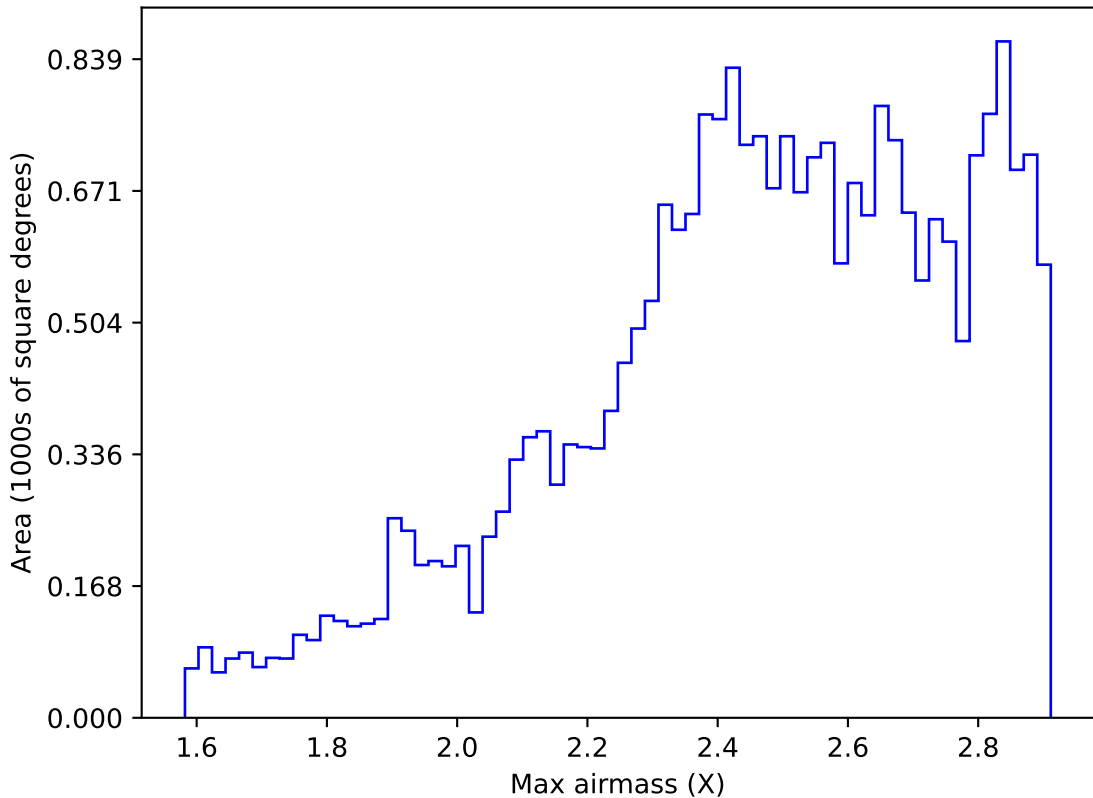
too_combined_no_nss_s10.0_v3.4_10yrs All sky z band: Max airmass
