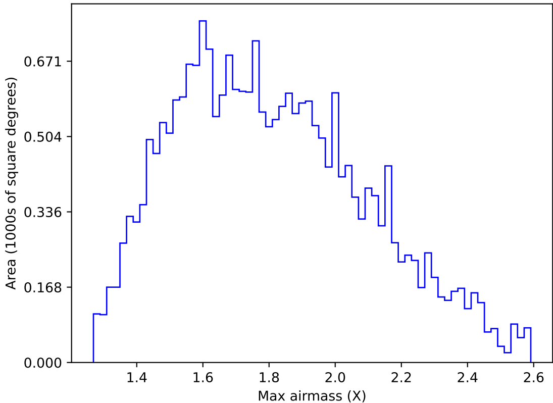
too_combined_no_nss_s10.0_v3.4_10yrs All sky u band: Max airmass
