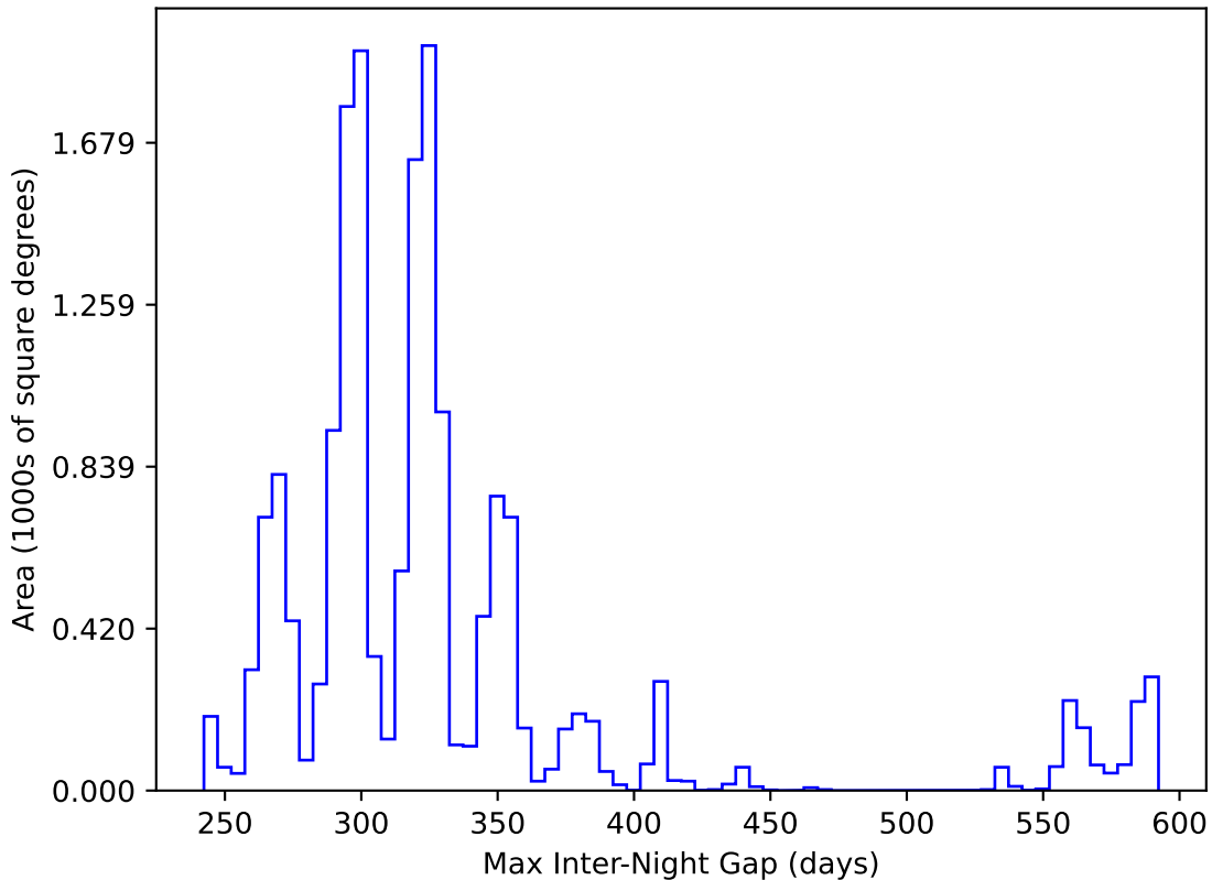
too_combined_no_nss_s10.0_v3.4_10yrs WFD y band: Max Inter-Night Gap
