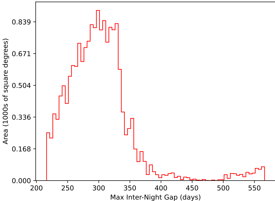
too_combined_no_nss_s10.0_v3.4_10yrs WFD i band: Max Inter-Night Gap
