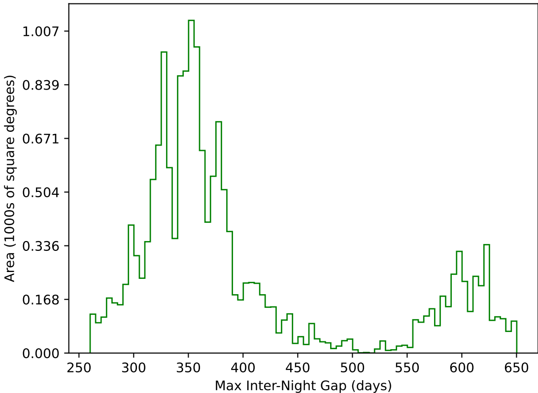
too_combined_no_nss_s10.0_v3.4_10yrs WFD g band: Max Inter-Night Gap
