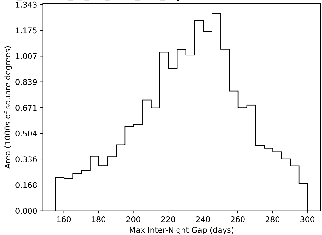
too_combined_no_nss_s10.0_v3.4_10yrs WFD all bands: Max Inter-Night Gap
