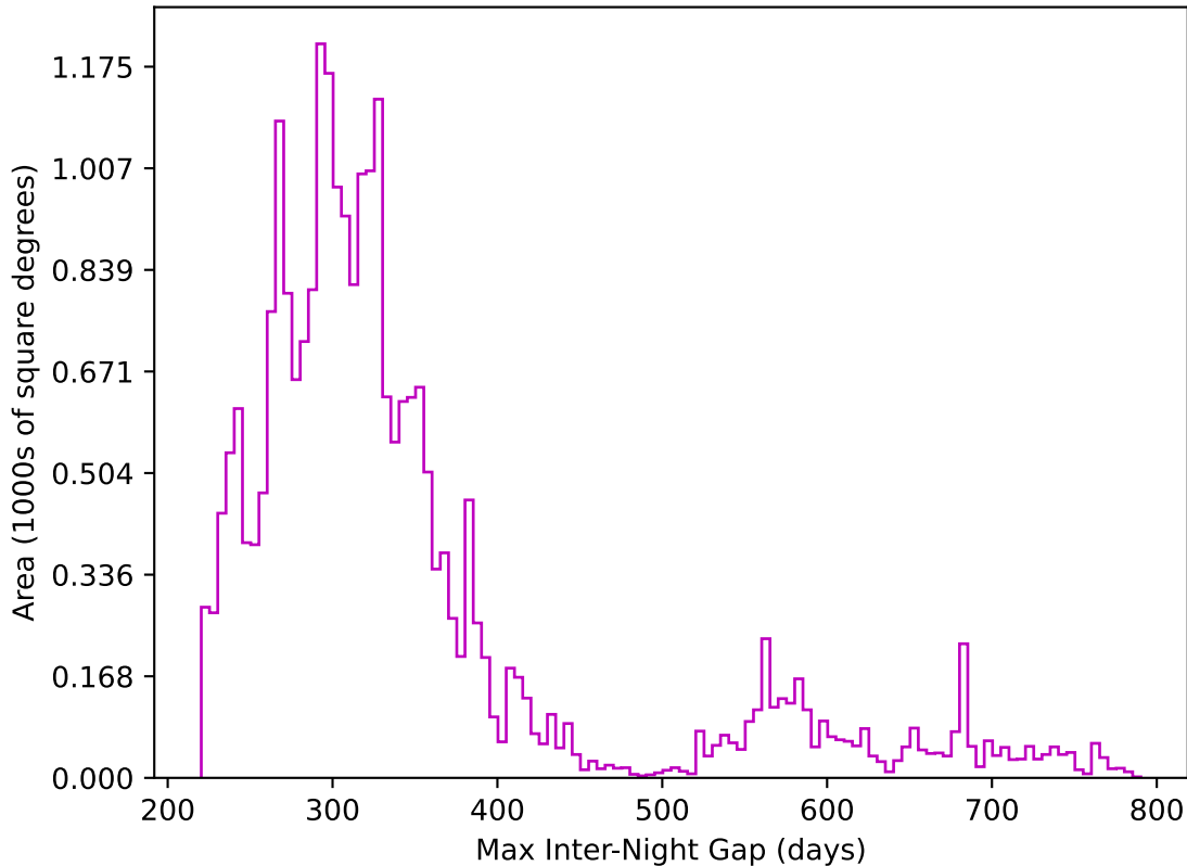
too_combined_no_nss_s10.0_v3.4_10yrs All sky z band: Max Inter-Night Gap
