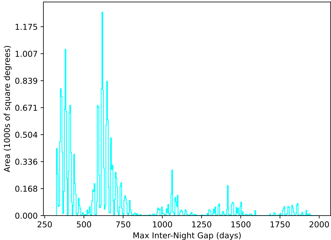
too_combined_no_nss_s10.0_v3.4_10yrs All sky u band: Max Inter-Night Gap
