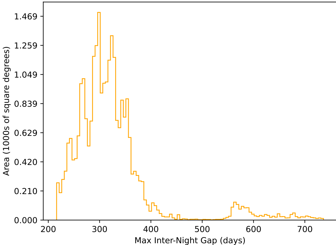
too_combined_no_nss_s10.0_v3.4_10yrs All sky r band: Max Inter-Night Gap
