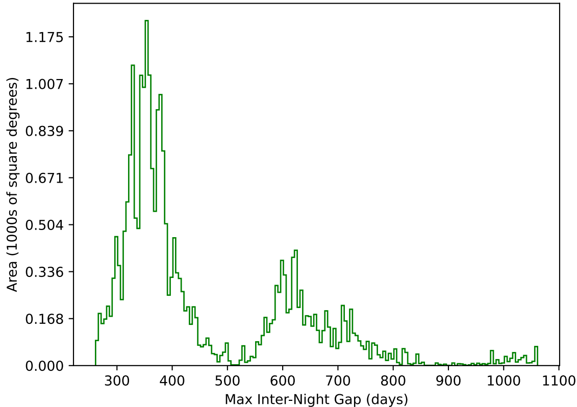
too_combined_no_nss_s10.0_v3.4_10yrs All sky g band: Max Inter-Night Gap
