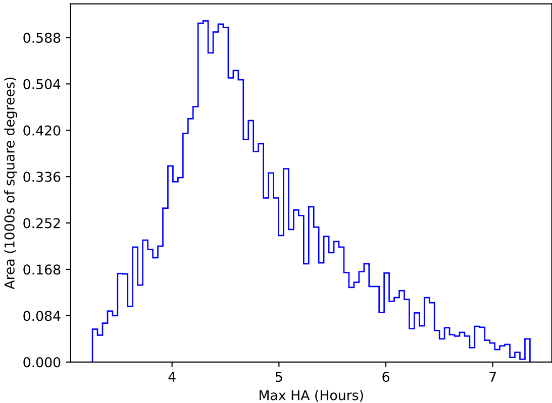
too_combined_no_nss_s10.0_v3.4_10yrs WFD y band: Max HA
