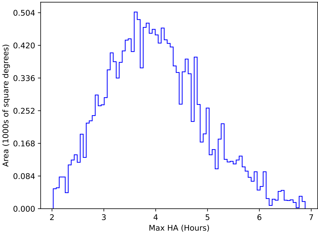
too_combined_no_nss_s10.0_v3.4_10yrs WFD u band: Max HA
