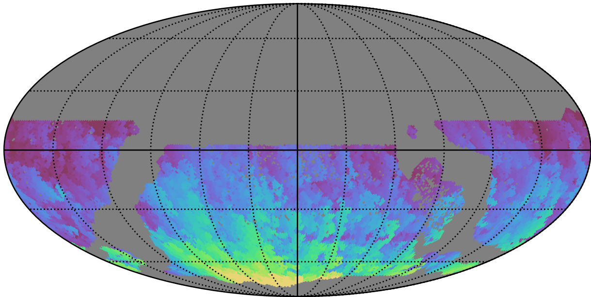
too_combined_no_nss_s10.0_v3.4_10yrs WFD r band: Max HA
