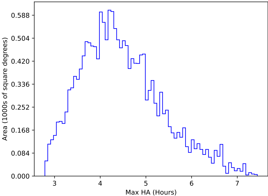
too_combined_no_nss_s10.0_v3.4_10yrs WFD r band: Max HA
