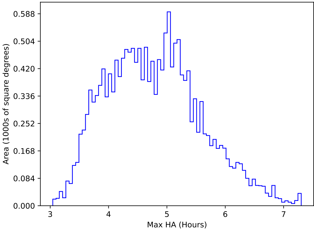
too_combined_no_nss_s10.0_v3.4_10yrs WFD i band: Max HA
