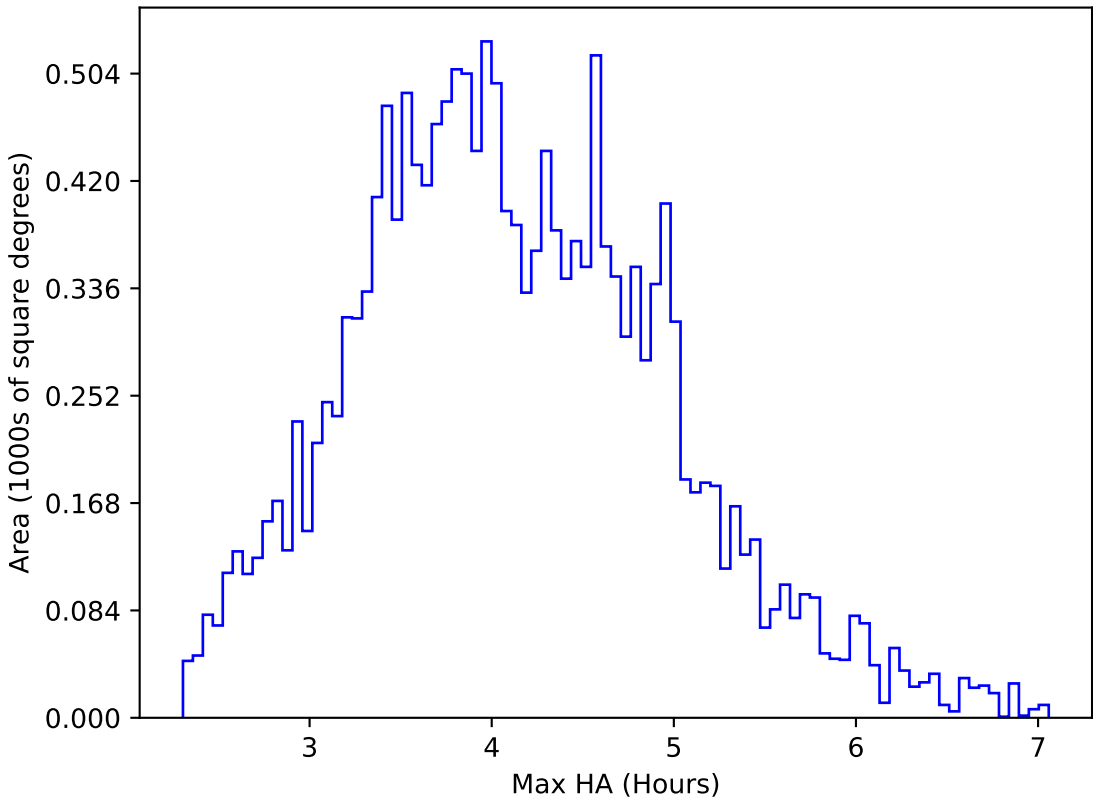
too_combined_no_nss_s10.0_v3.4_10yrs WFD g band: Max HA
