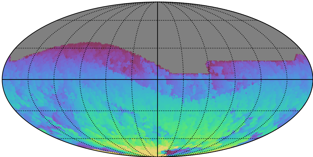
too_combined_no_nss_s10.0_v3.4_10yrs All sky z band: Max HA
