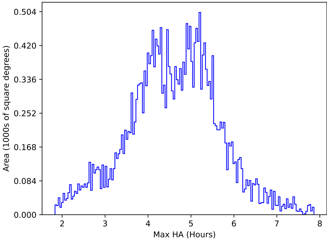
too_combined_no_nss_s10.0_v3.4_10yrs All sky z band: Max HA
