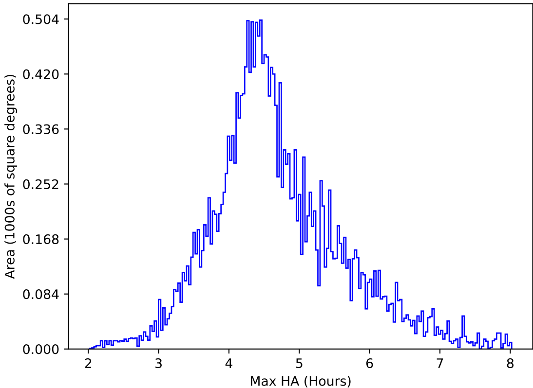
too_combined_no_nss_s10.0_v3.4_10yrs All sky y band: Max HA
