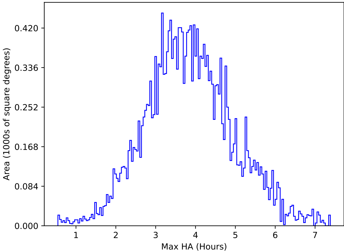
too_combined_no_nss_s10.0_v3.4_10yrs All sky u band: Max HA
