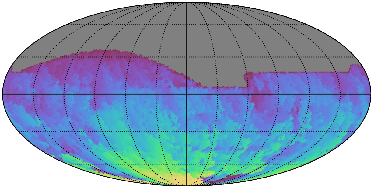
too_combined_no_nss_s10.0_v3.4_10yrs All sky r band: Max HA
