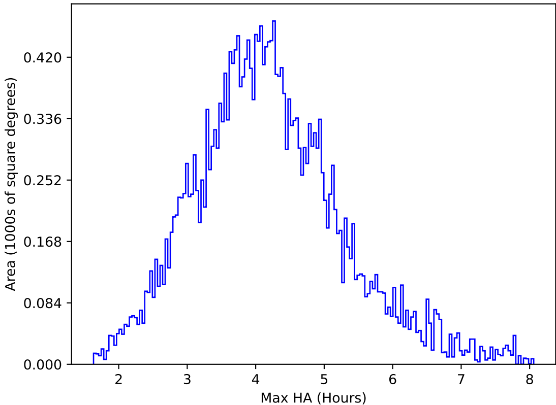
too_combined_no_nss_s10.0_v3.4_10yrs All sky r band: Max HA
