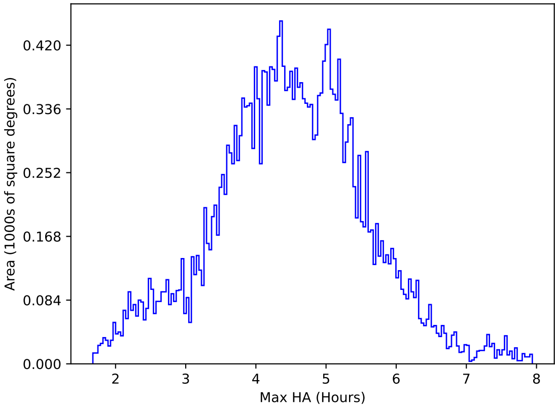
too_combined_no_nss_s10.0_v3.4_10yrs All sky i band: Max HA
