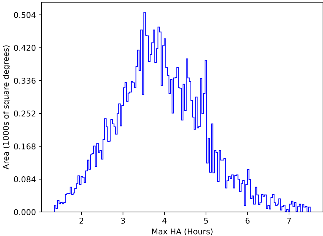
too_combined_no_nss_s10.0_v3.4_10yrs All sky g band: Max HA
