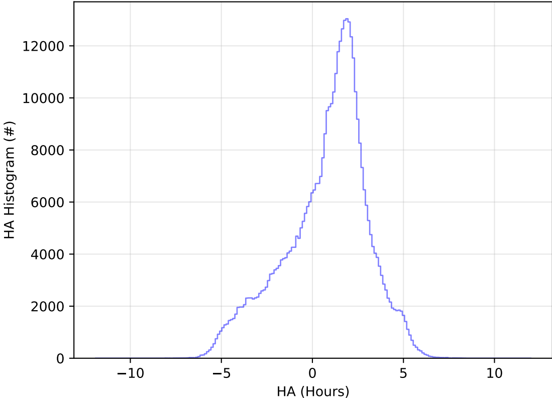
too_combined_no_nss_s10.0_v3.4_10yrs WFD z band: HA Histogram
