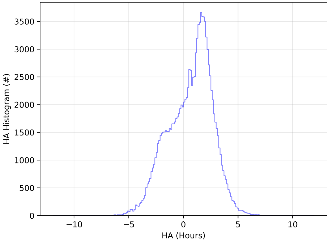
too_combined_no_nss_s10.0_v3.4_10yrs WFD u band: HA Histogram
