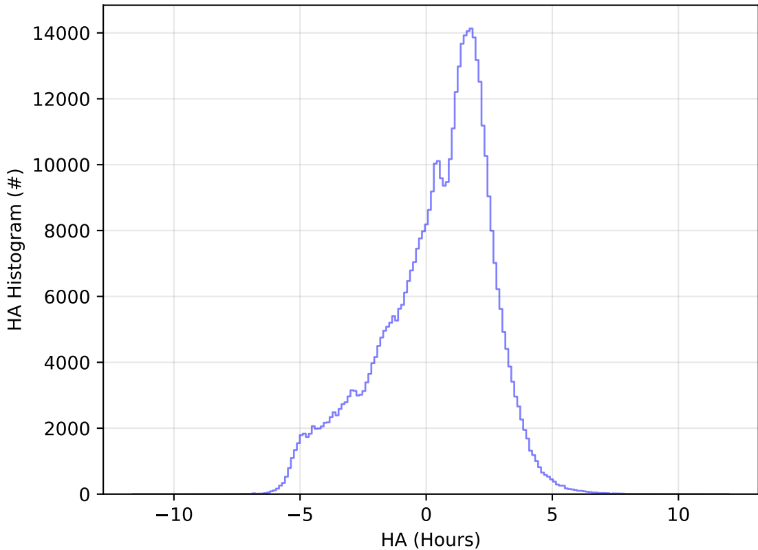
too_combined_no_nss_s10.0_v3.4_10yrs WFD r band: HA Histogram
