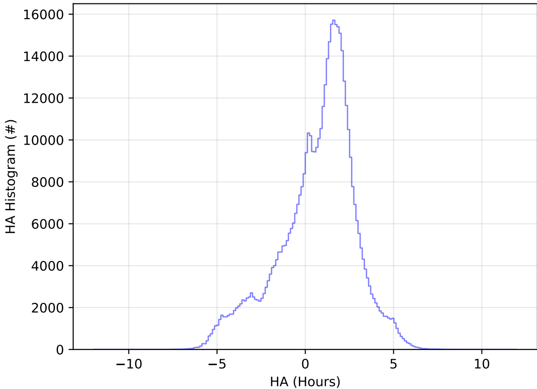
too_combined_no_nss_s10.0_v3.4_10yrs WFD i band: HA Histogram
