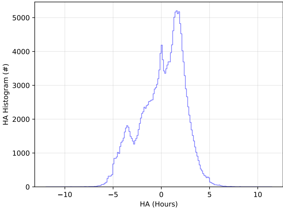
too_combined_no_nss_s10.0_v3.4_10yrs WFD g band: HA Histogram
