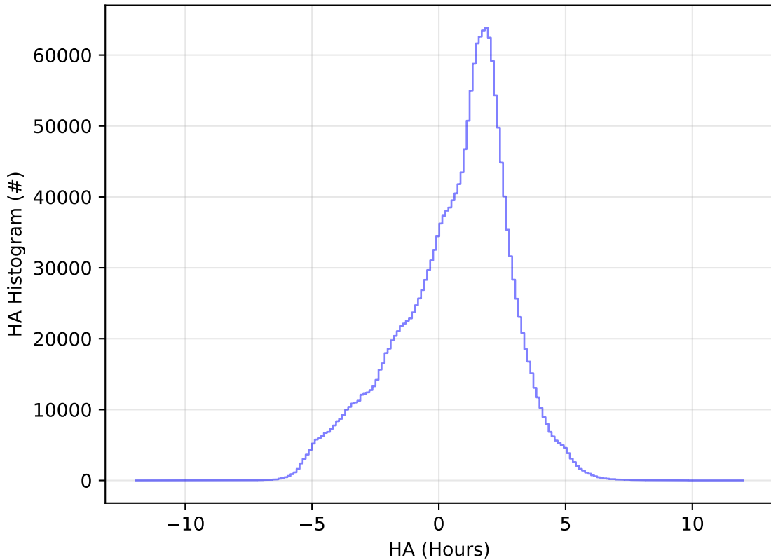
too_combined_no_nss_s10.0_v3.4_10yrs WFD all bands: HA Histogram
