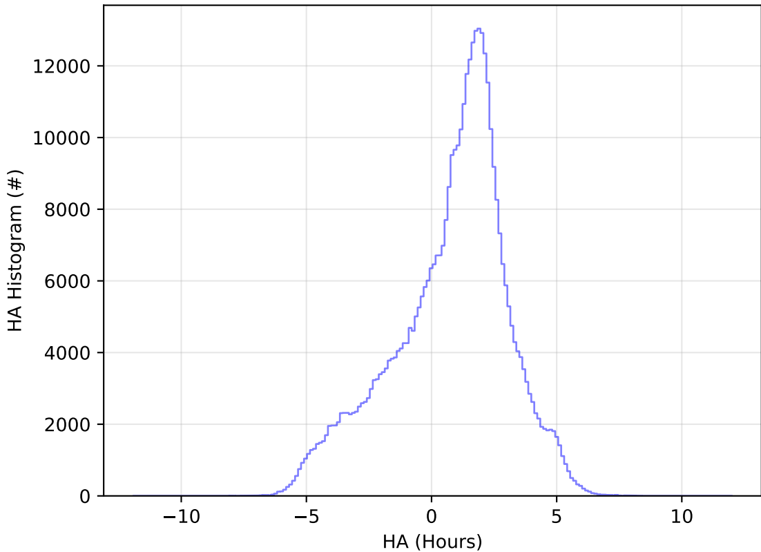
too_combined_no_nss_s10.0_v3.4_10yrs All sky z band: HA Histogram
