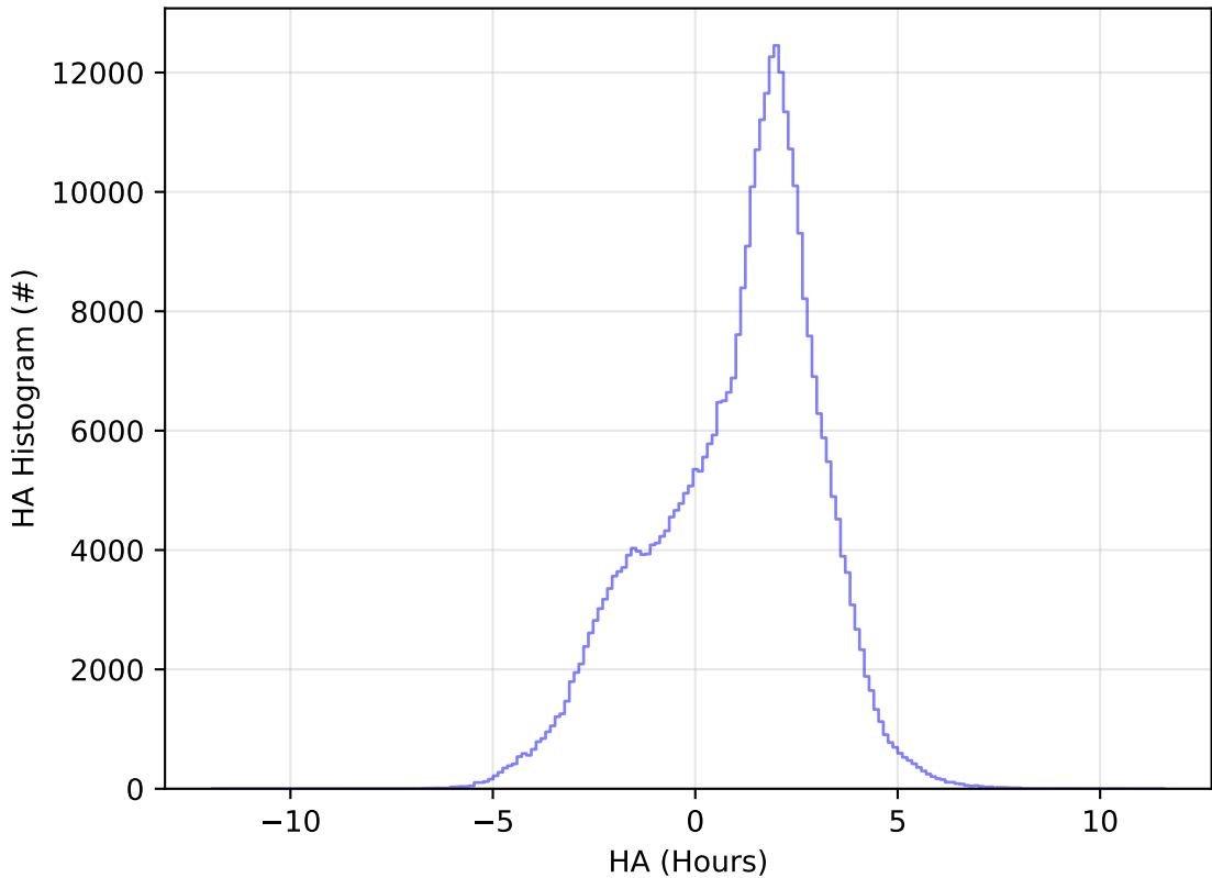
too_combined_no_nss_s10.0_v3.4_10yrs All sky y band: HA Histogram
