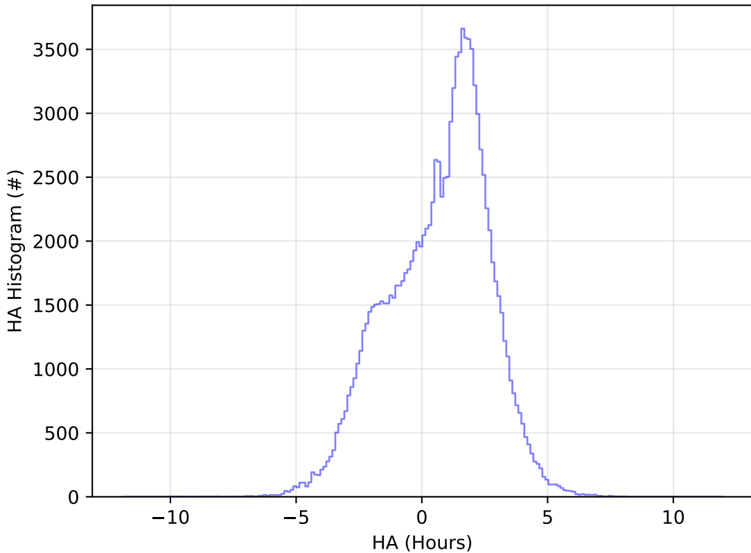
too_combined_no_nss_s10.0_v3.4_10yrs All sky u band: HA Histogram
