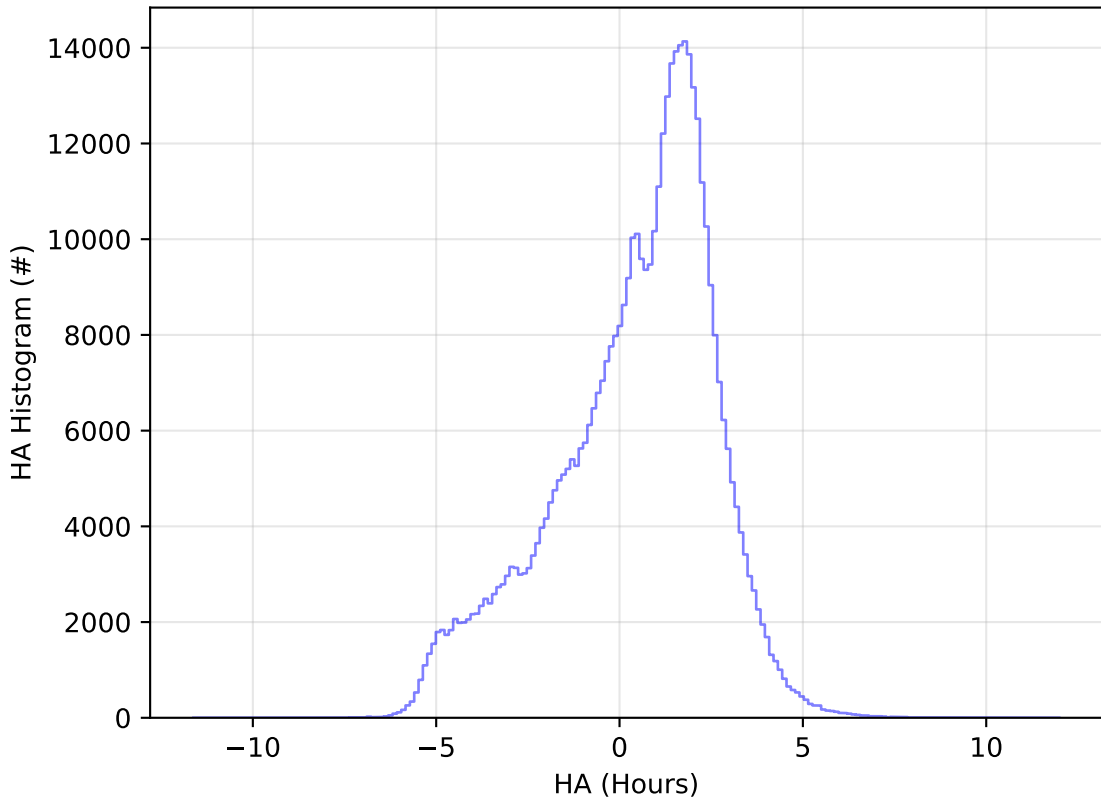
too_combined_no_nss_s10.0_v3.4_10yrs All sky r band: HA Histogram
