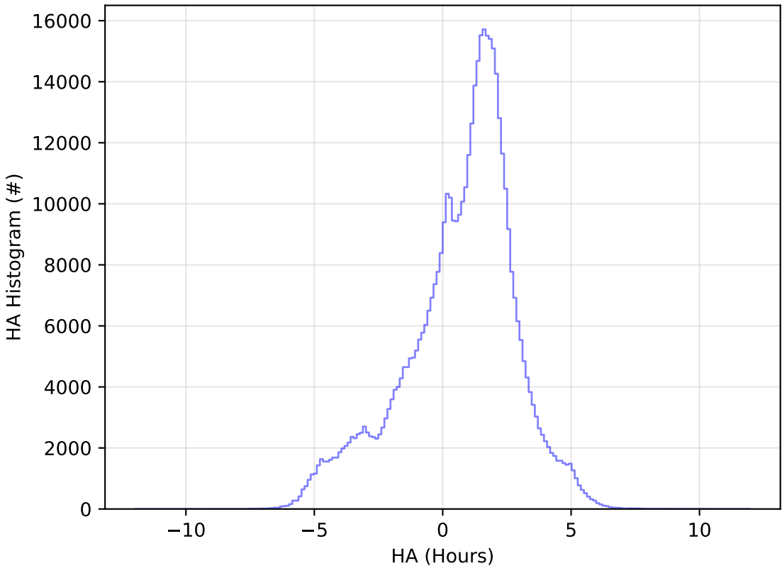
too_combined_no_nss_s10.0_v3.4_10yrs All sky i band: HA Histogram
