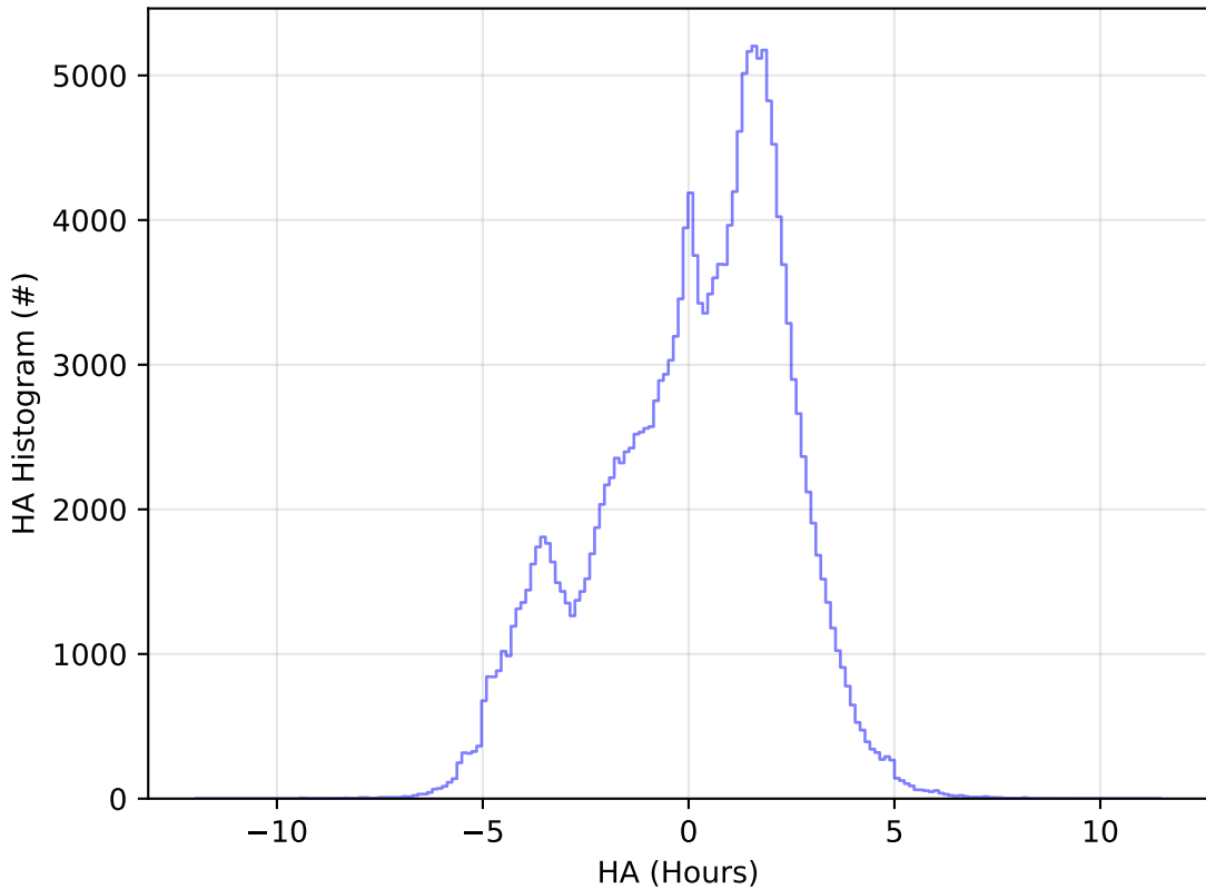
too_combined_no_nss_s10.0_v3.4_10yrs All sky g band: HA Histogram
