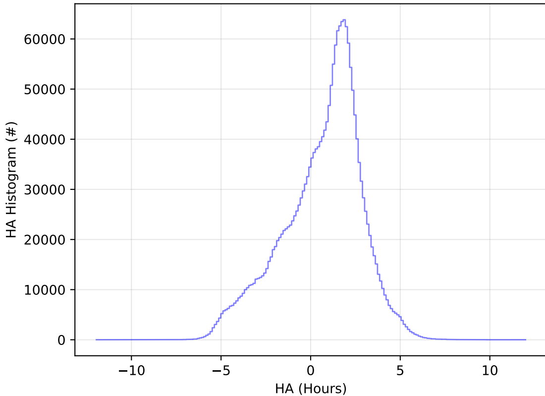
too_combined_no_nss_s10.0_v3.4_10yrs All sky all bands: HA Histogram
