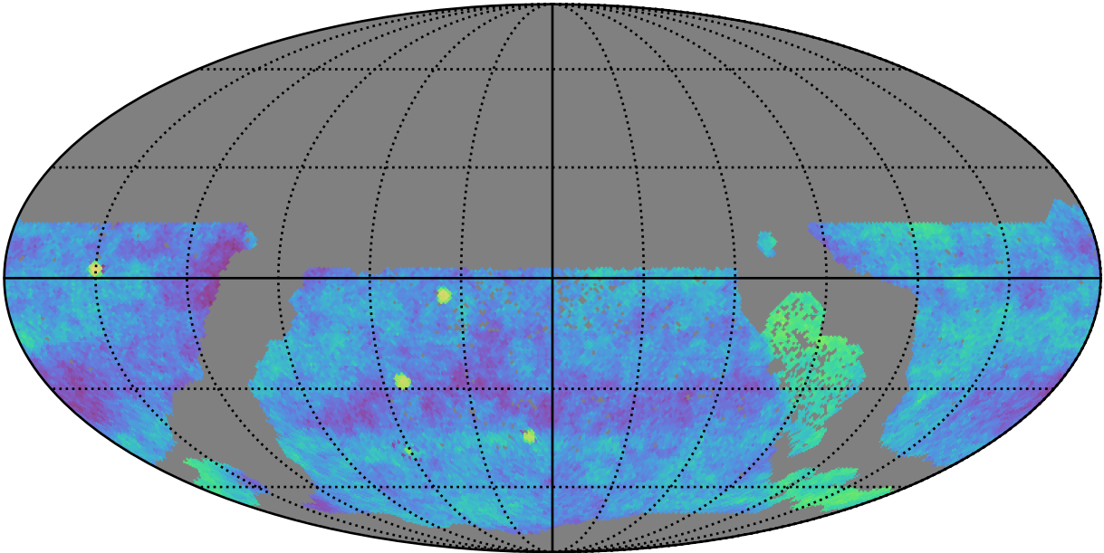
too_combined_no_nss_s10.0_v3.4_10yrs gri WFD: Fraction of visits in pairs (20-90 min)
