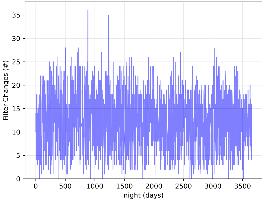
too_combined_no_nss_s10.0_v3.4_10yrs Per Night: Filter Changes
