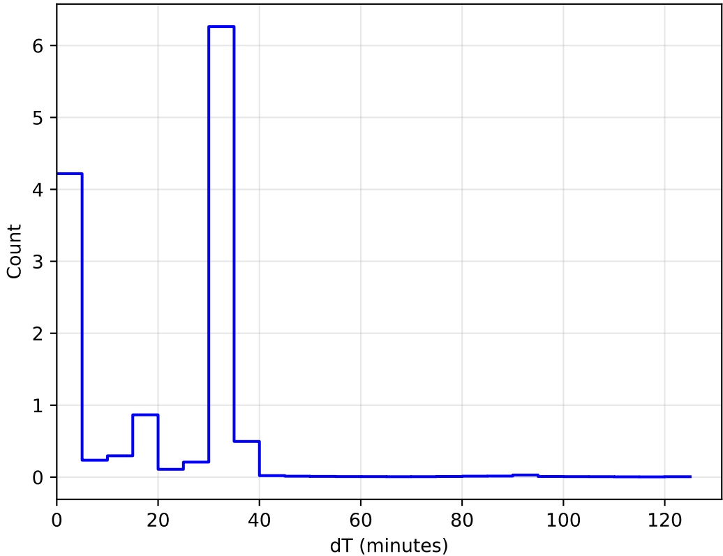
too_combined_no_nss_s10.0_v3.4_10yrs All sky: DeltaT Histogram
