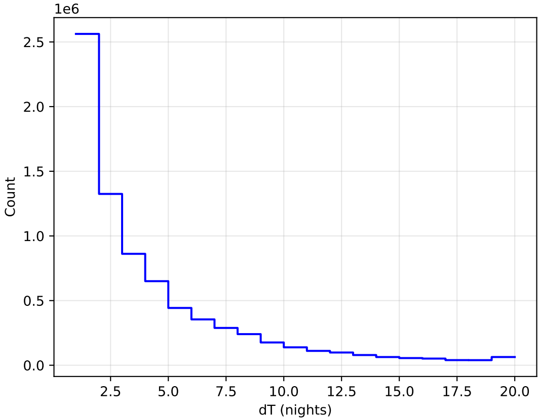
too_combined_no_nss_s10.0_v3.4_10yrs WFD all bands: DeltaNight Histogram
