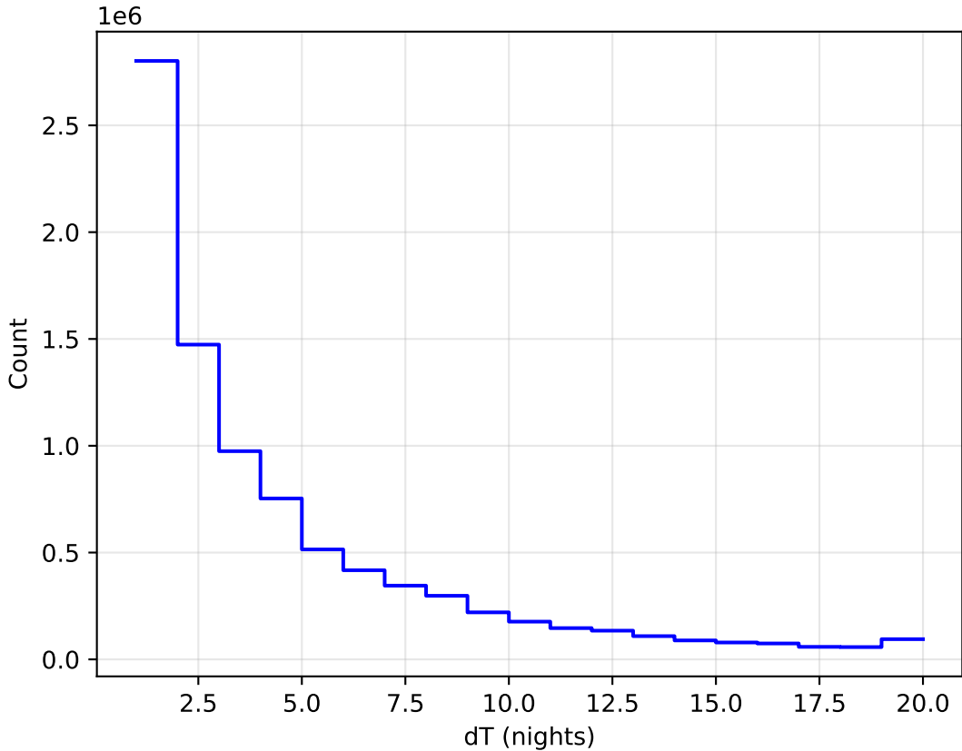
too_combined_no_nss_s10.0_v3.4_10yrs All sky all bands: DeltaNight Histogram
