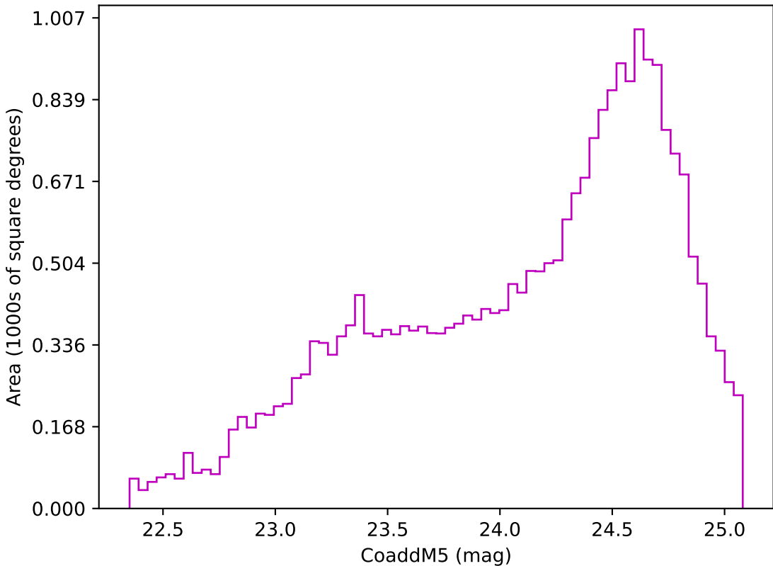
too_combined_no_nss_s10.0_v3.4_10yrs Yr 3-4 z band: CoaddM5
