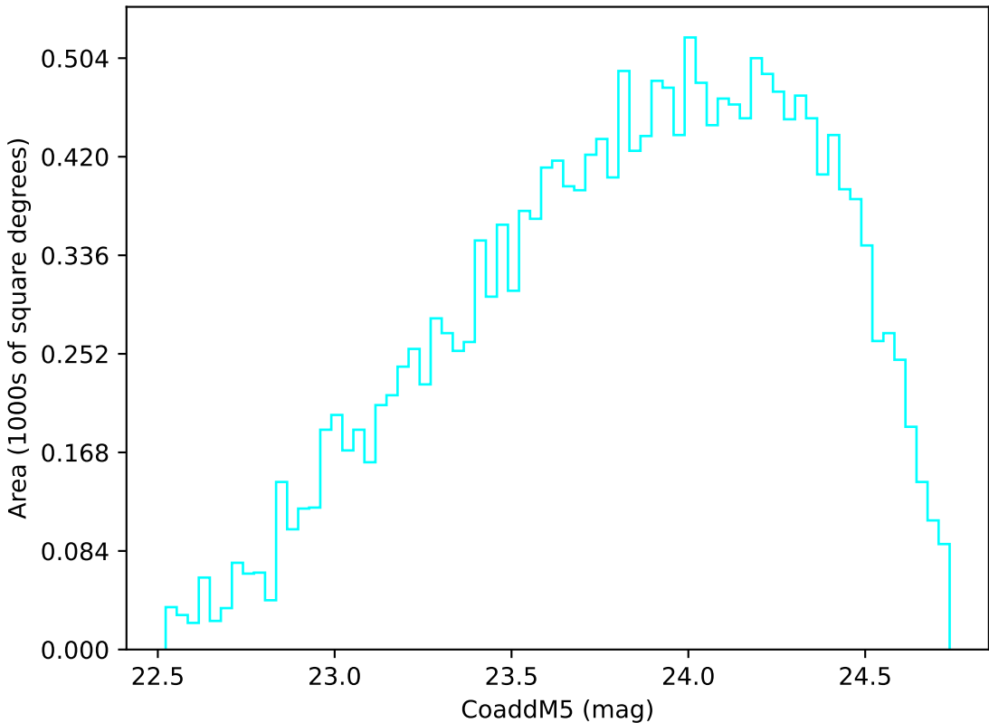
too_combined_no_nss_s10.0_v3.4_10yrs Yr 3-4 u band: CoaddM5
