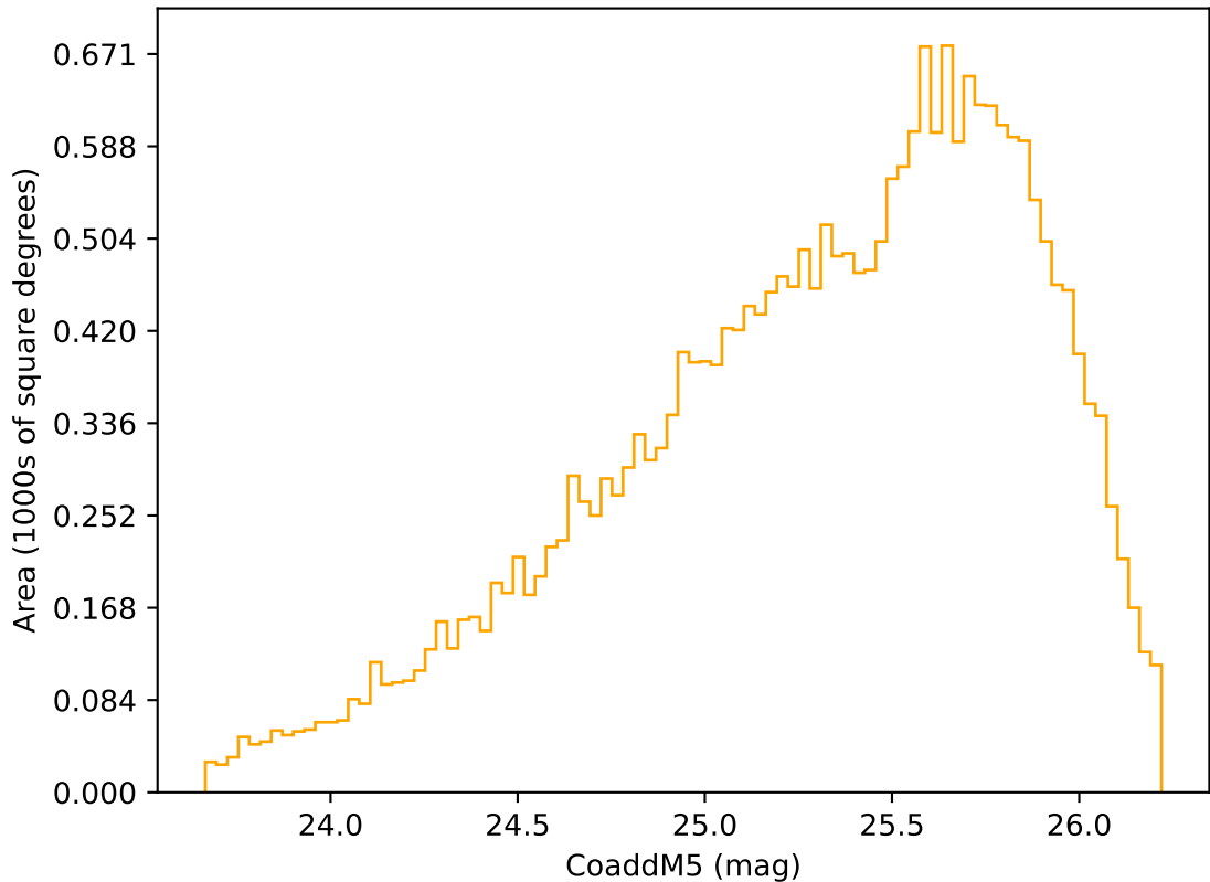
too_combined_no_nss_s10.0_v3.4_10yrs Yr 3-4 r band: CoaddM5
