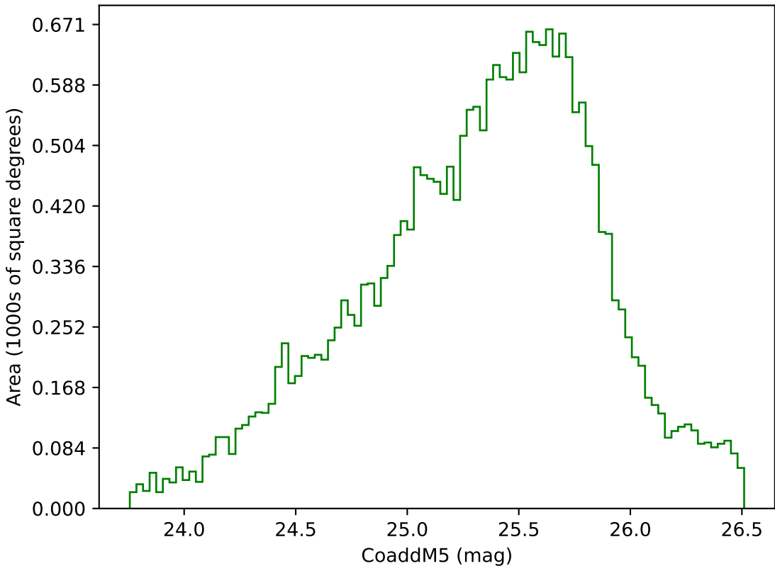
too_combined_no_nss_s10.0_v3.4_10yrs Yr 3-4 g band: CoaddM5
