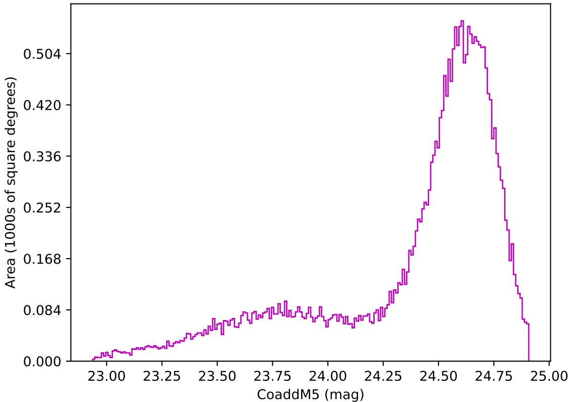
too_combined_no_nss_s10.0_v3.4_10yrs Yr 1 z band: CoaddM5
