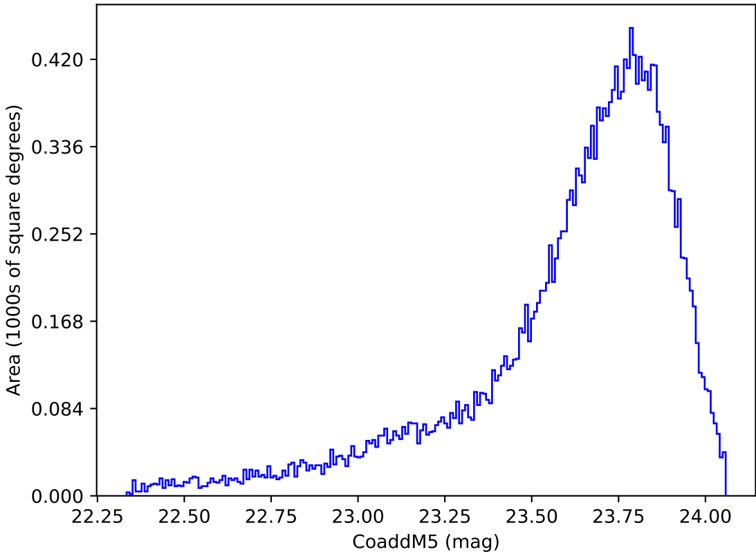
too_combined_no_nss_s10.0_v3.4_10yrs Yr 1 y band: CoaddM5
