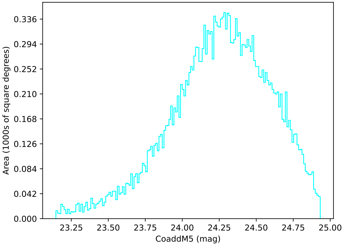
too_combined_no_nss_s10.0_v3.4_10yrs Yr 1 u band: CoaddM5
